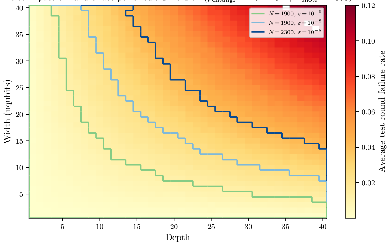
Noise impact on failure rate per circuit dimension ( p_{\text{entangle}} = 1.5 \times 10^{-5} , N_{\text{shots}} = 1000 )
