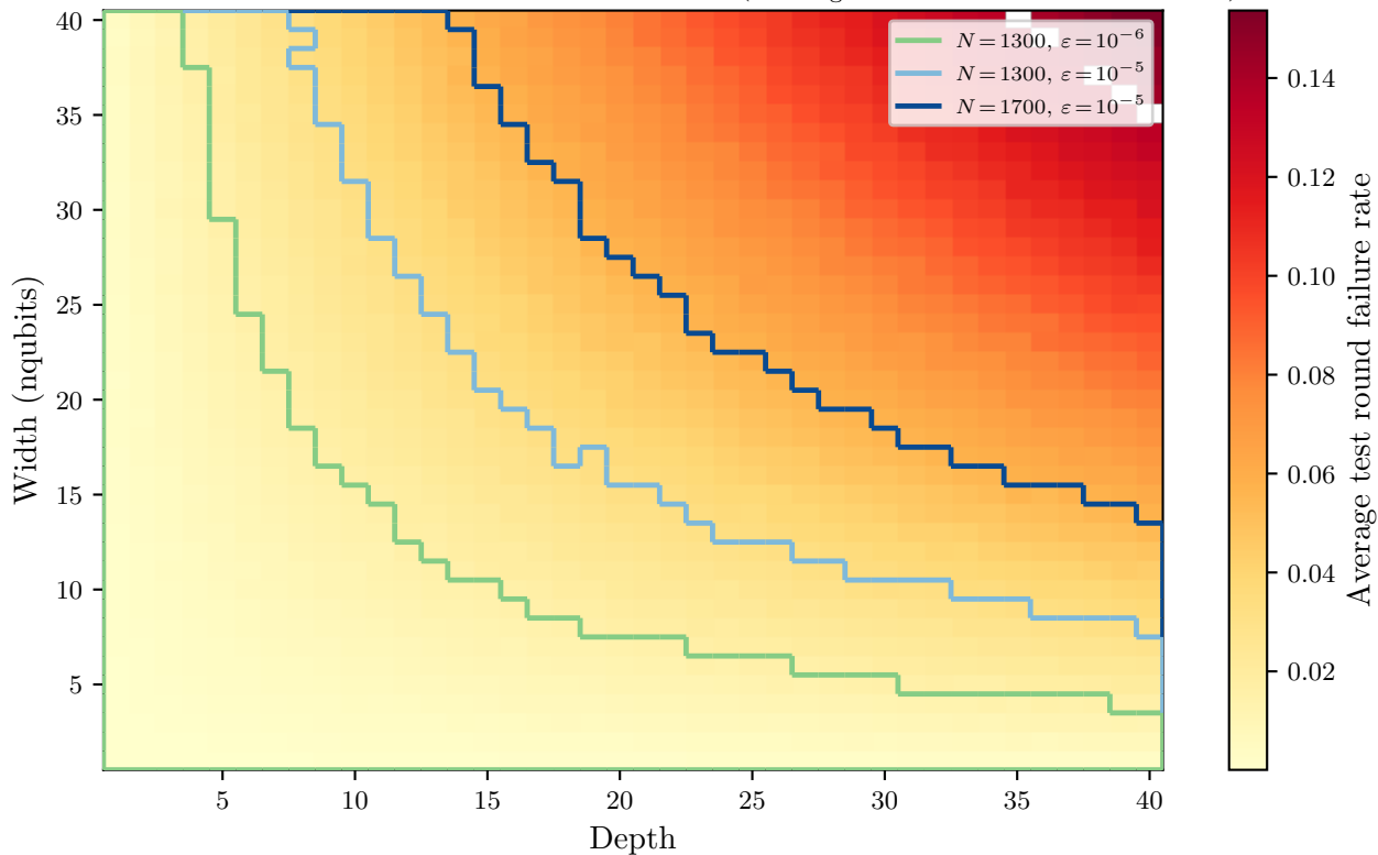
Noise impact on failure rate per circuit dimension ( p_{\text{entangle}} = 2 \times 10^{-5} , N_{\text{shots}} = 1000 )
