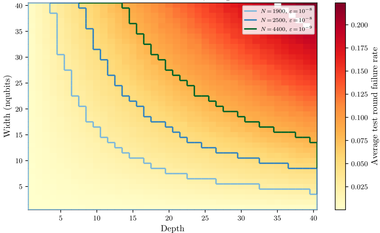
Noise impact on failure rate per circuit dimension ( p_{\text{entangle}} = 3 \times 10^{-5} , N_{\text{shots}} = 1000 )
