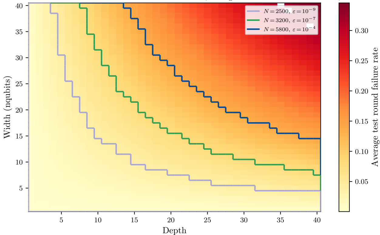
Noise impact on failure rate per circuit dimension ( p_{\text{entangle}} = 5 \times 10^{-5} , N_{\text{shots}} = 1000 )
