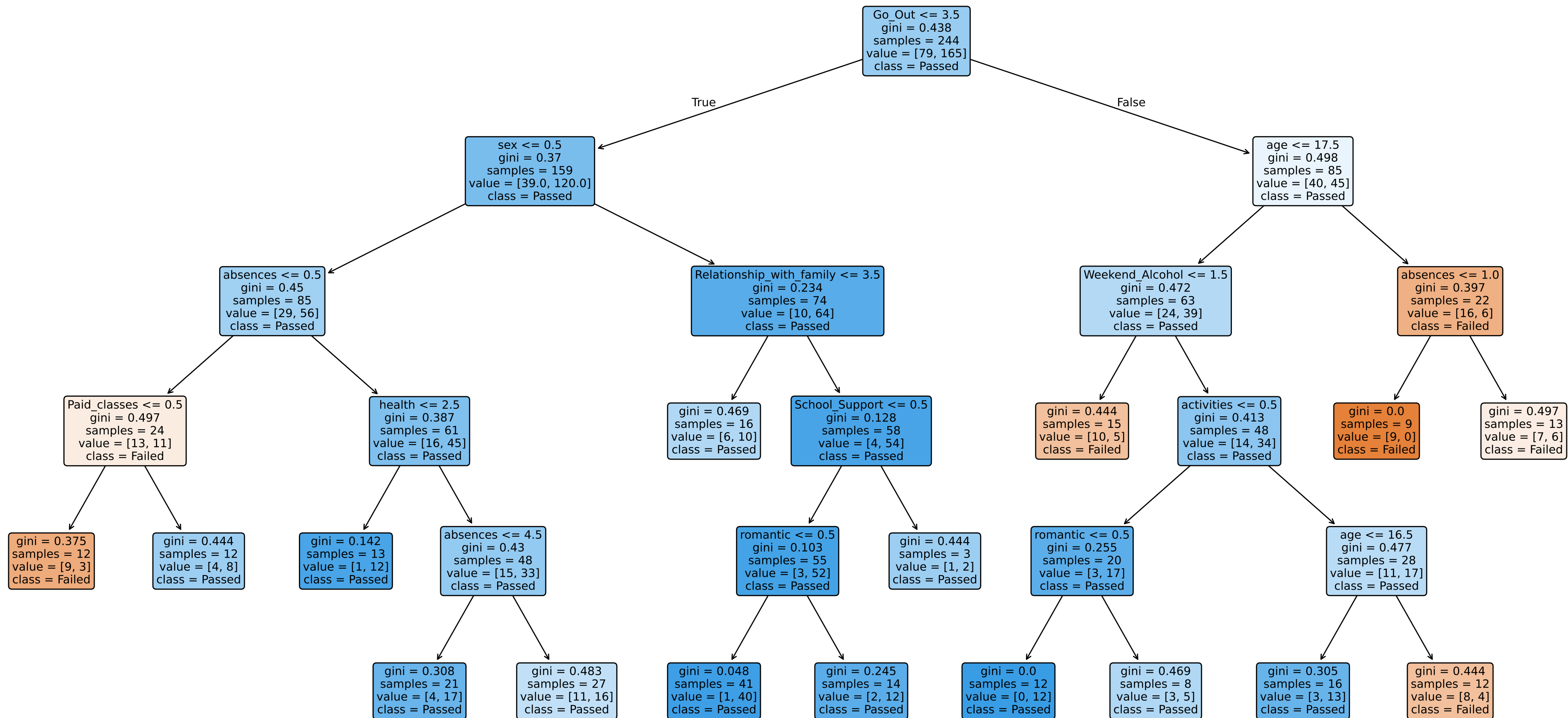
Decision Tree for Student Success Prediction (max_depth=5)
