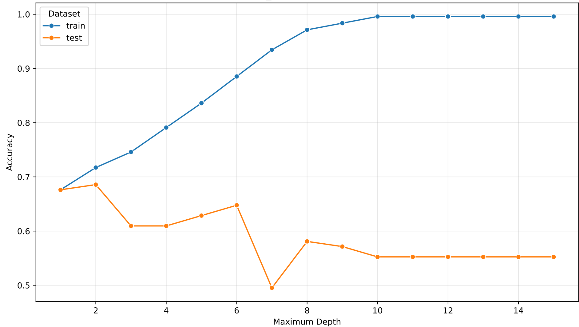
Effect of max_depth on Model Performance
