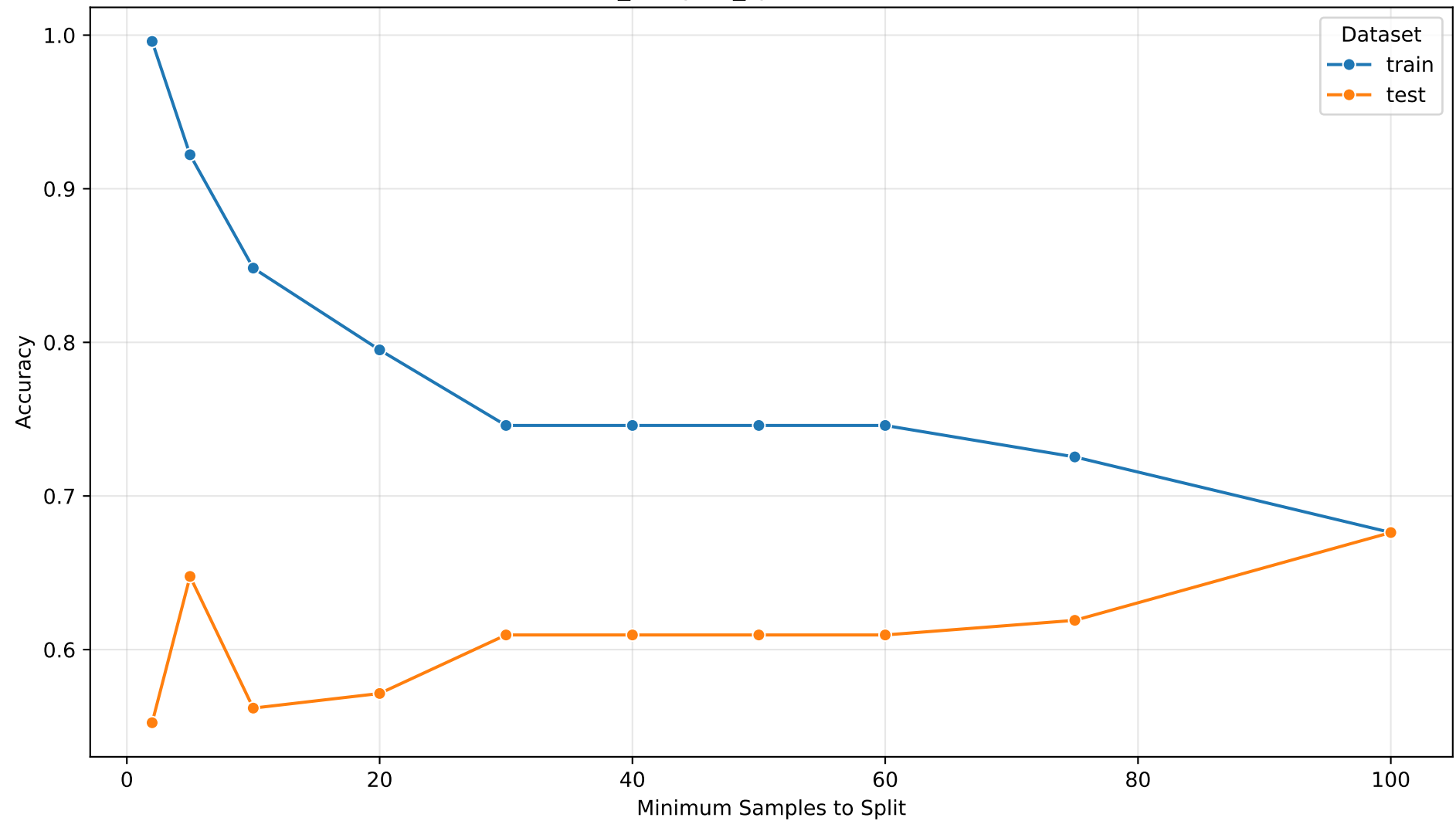
Effect of min_samples_split on Model Performance
