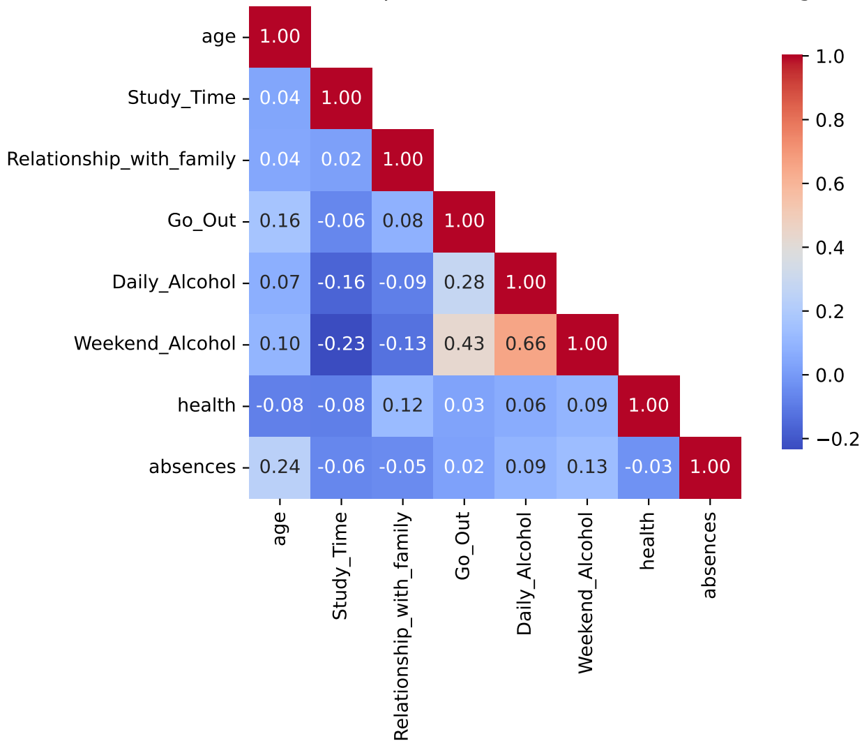
Correlation Heatmap - Numeric Variables (Lower Triangle)
