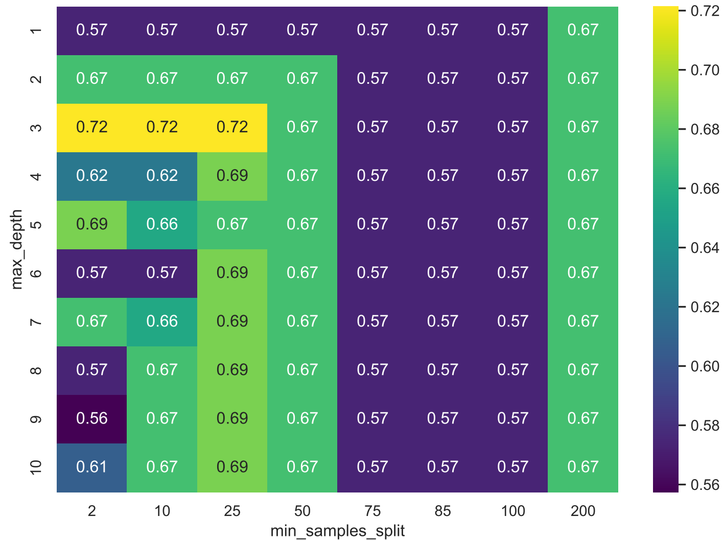
Grid Search Results - Decision Tree Classifier
