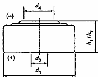
Figure 12 – Dessins des dimensions: SR62, SR63, SR65, SR64, SR60, SR67, SR66, SR58, SR68, SR59, SR69, SR41, SR57, SR55, SR48, SR54, SR42, SR43, SR44
