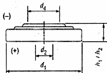
Figure 13 - Dessins des dimensions: CR1025, CR1216, CR1220, CR1616, CR2012, CR1620, CR2016, CR2025, CR2320, CR2032, CR2330, CR2430, CR2354, CR3032, CR2450, BR1225, BR2016, BR2320, BR2325, BR3032
