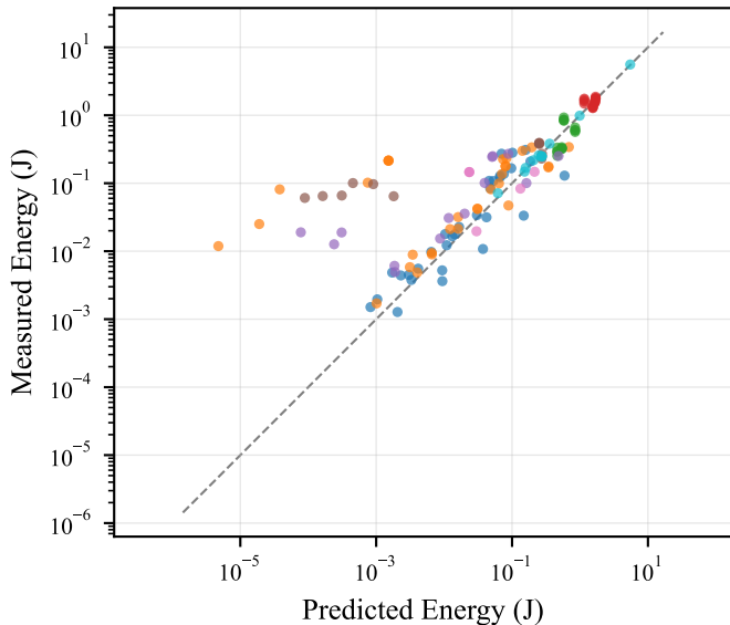
RTX 4090 ( r^2 = 0.947 )
