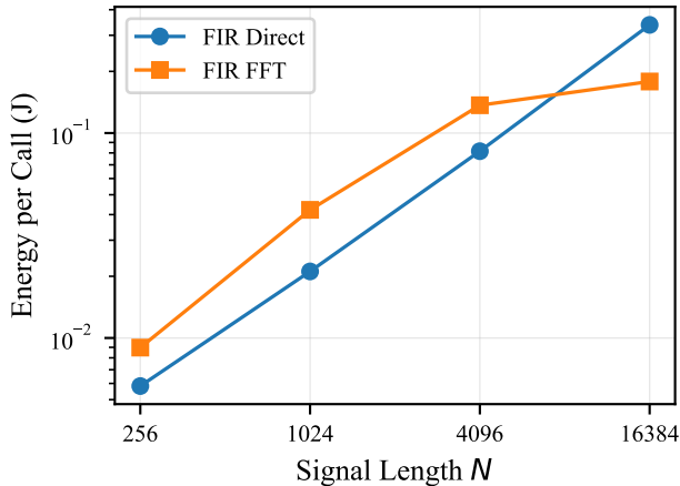
FIR Direct vs. FFT-based Convolution
