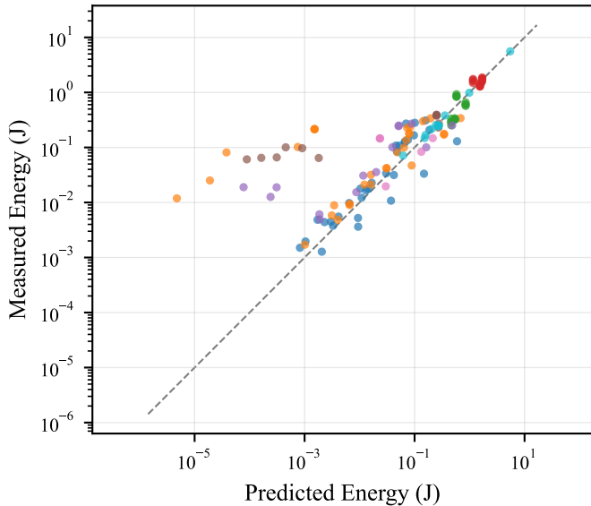
RTX 4090 Laptop ( r^2 = 0.947 )
