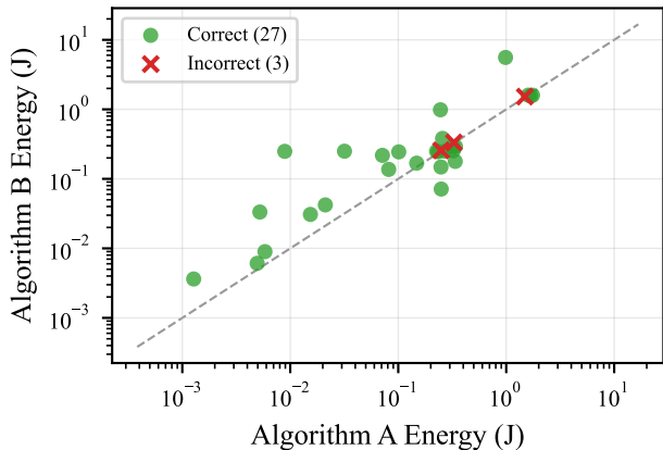
Head-to-Head Ranking, RTX 4090 (27/30)
