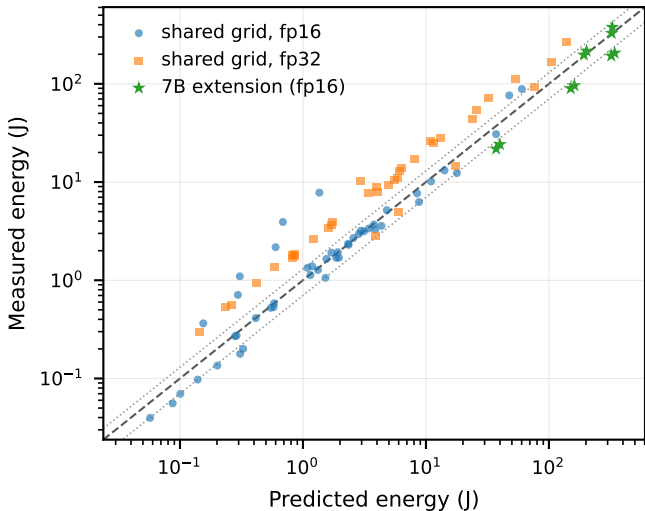
A100, M8 fitted on the 84 shared points in-sample MAPE 35.8%, 7B extrapolation 42.7%
