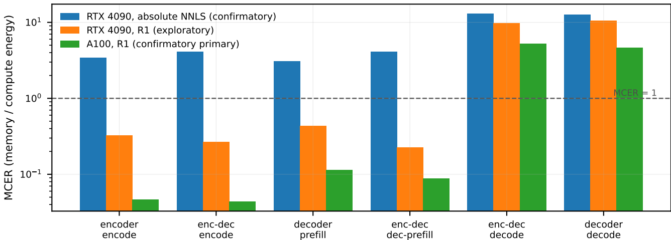
Prefill and decode separate by 4x to 40x on both platforms; the crossing of unity is estimator dependent
