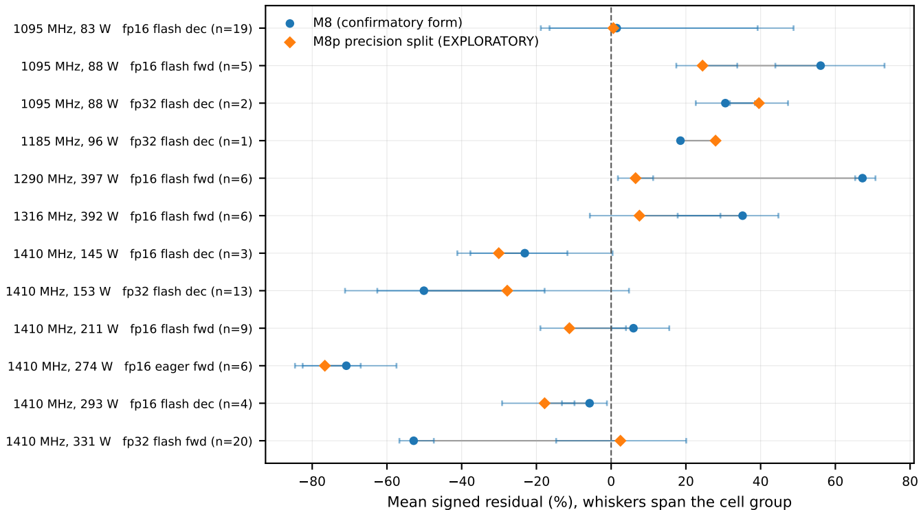
Residual by operating point and execution path (rows ordered by SM clock; whiskers are min to max)
