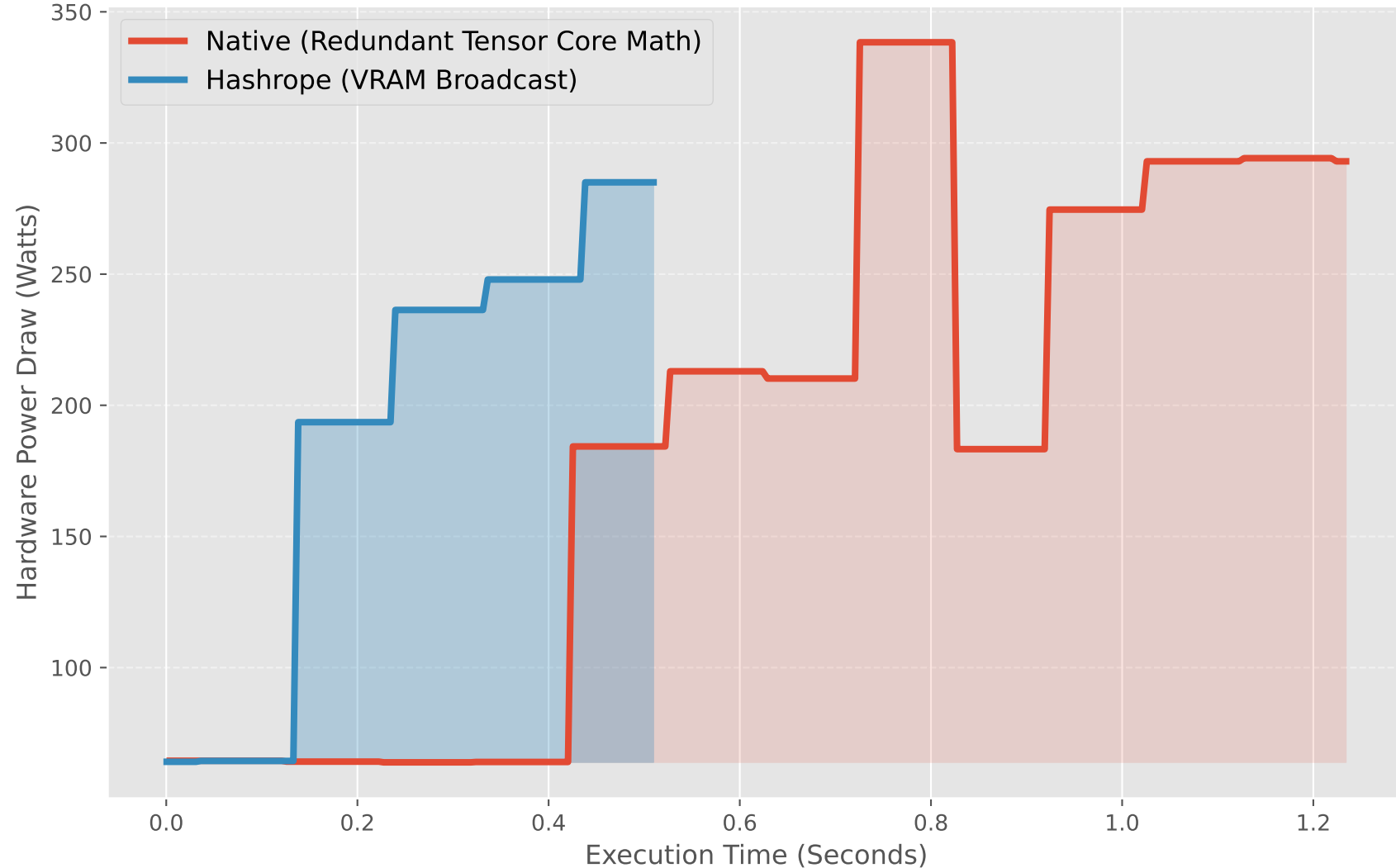
A100 GPU Power Envelope (Wattage over Time)
