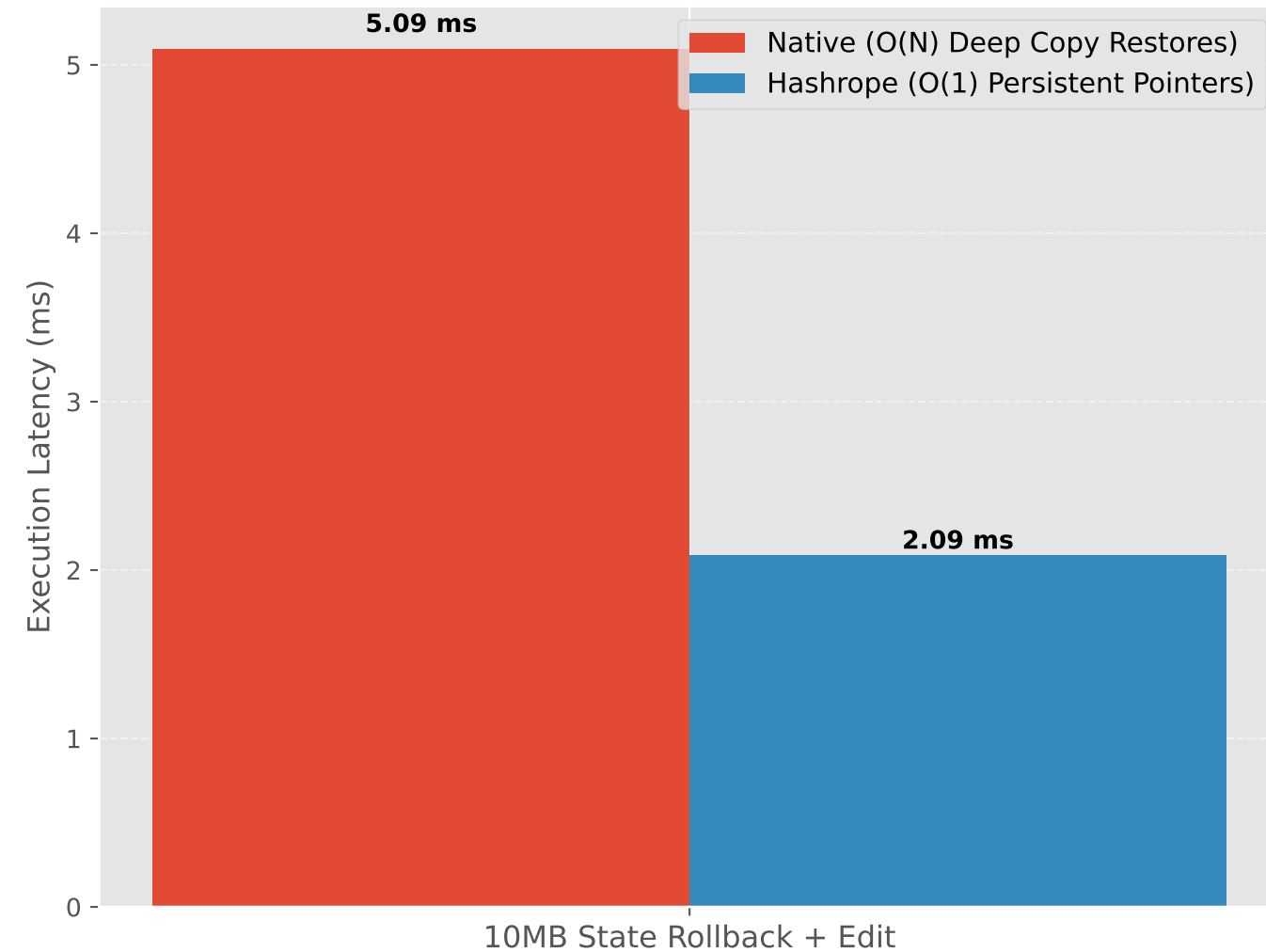
Agentic Time-Travel (Rollbacks)
