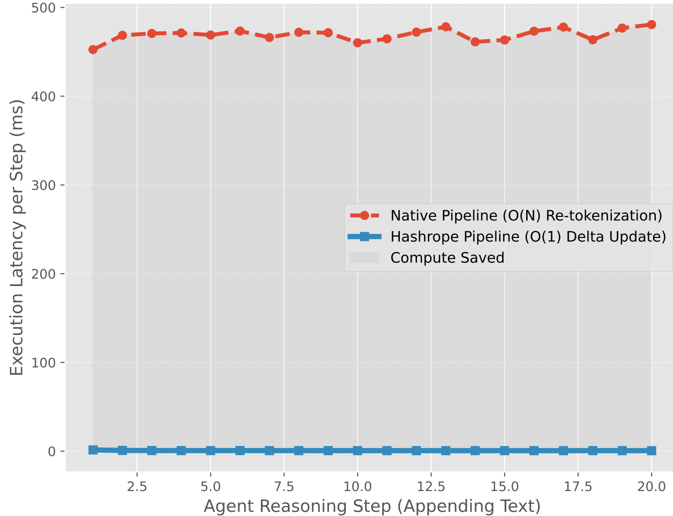
Agentic ReAct Loop: Delta-Tokenization
