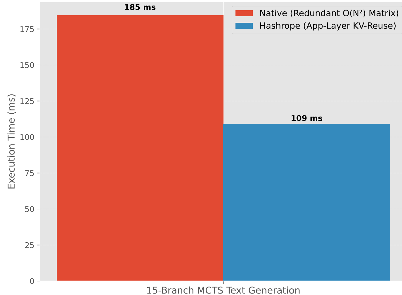
End-to-End LLM Generation Synergy
