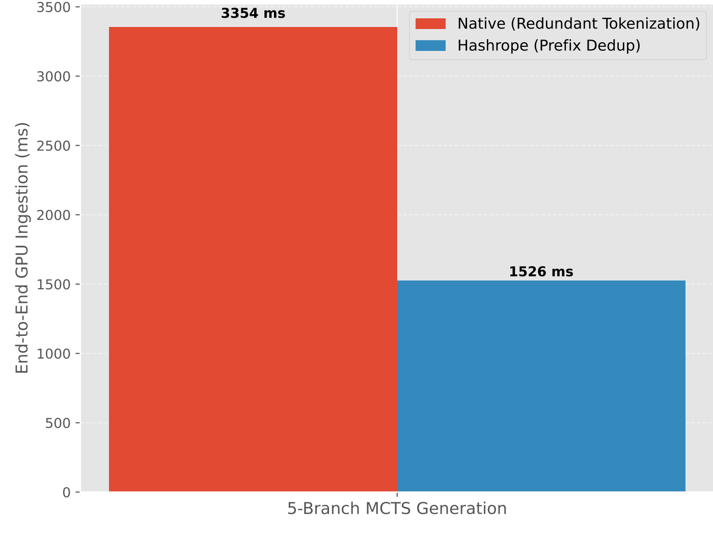
App-Layer Prefix Caching (Tree of Thoughts)
