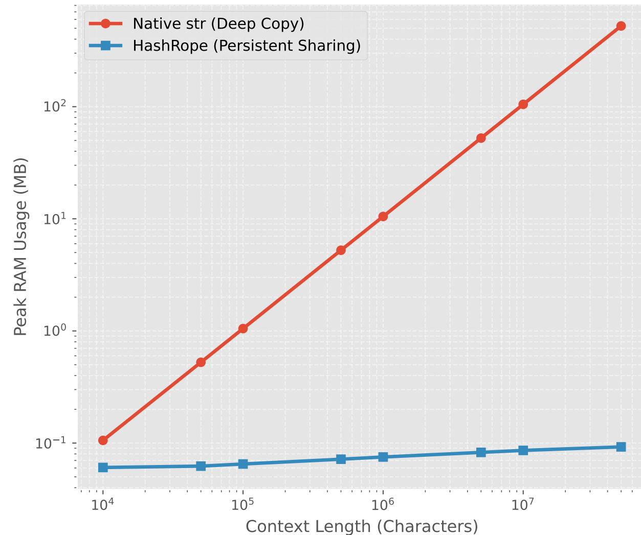
Agent Tree-of-Thoughts Forking (10 Branches)
