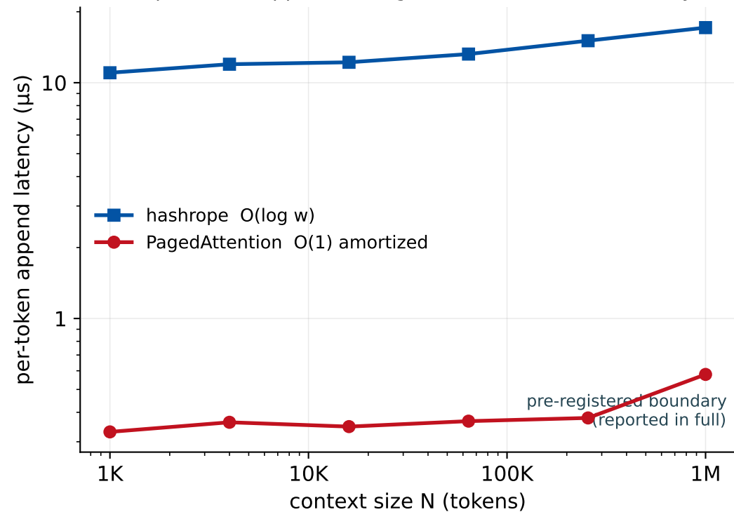
(a) per-token append — PagedAttention wins (boundary)
