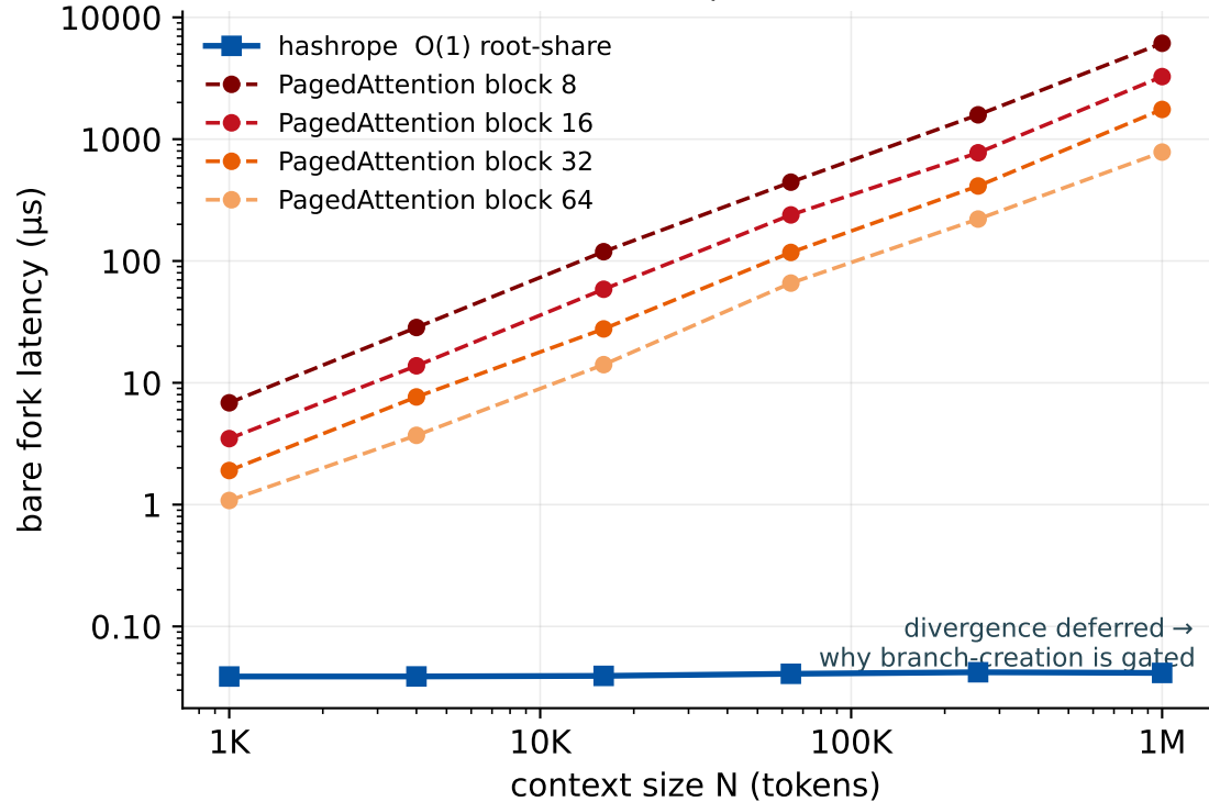
(b) bare fork — hashrope O(1), no crossover
