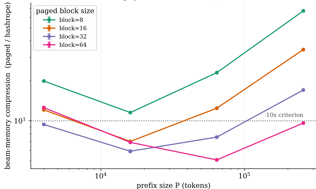
EXP-019 Milestone B: beam-memory compression on real ToT beams ( \leq 5 survivors) 17x-67x across deployment-standard blocks {8,16,32} at P=256k
