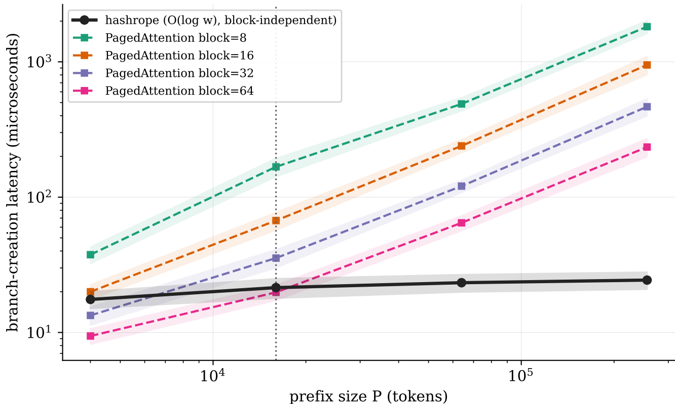
EXP-019 Milestone B: branch-creation latency on real Game-of-24 ToT traces hashrope flat ( O(\log w) ); PagedAttention linear ( O(\text{ceil}(N/B)) ); block-dependent crossover
