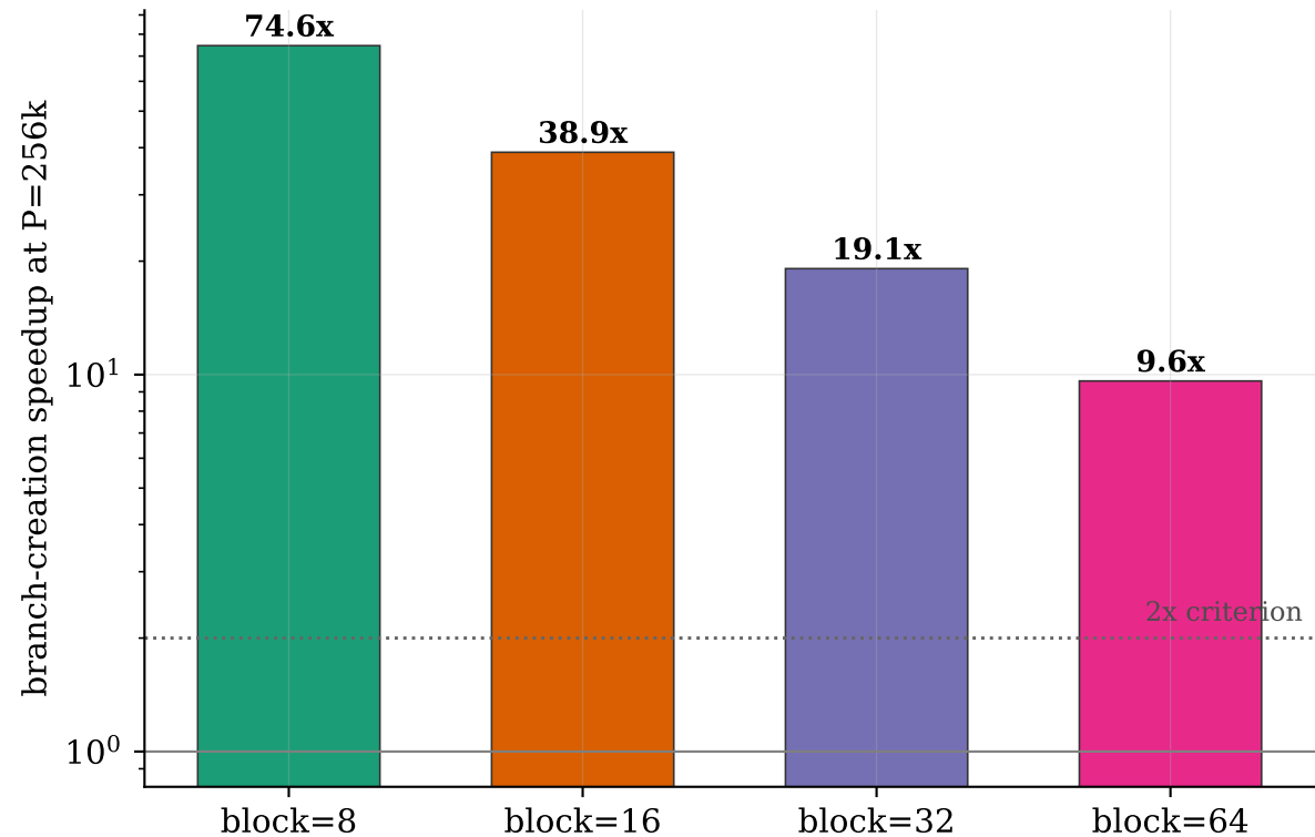
EXP-019 Milestone B: branch-creation speedup at P=256k 9/9 paired wins at every block (n=9)
