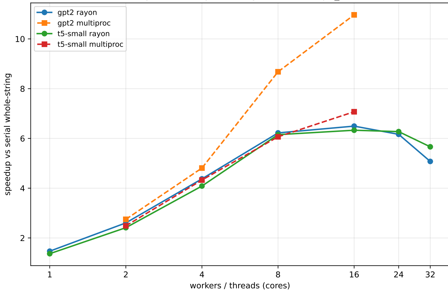
EXP-001: rayon vs multiprocessing @ 4096KB (cpu_count=32)
