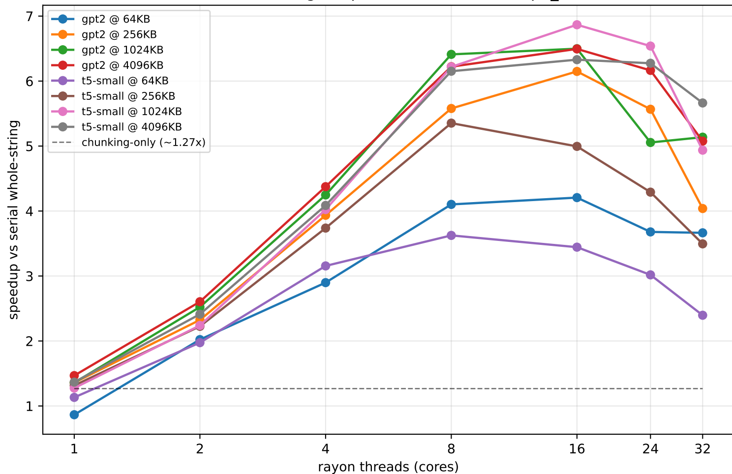
EXP-001: tokenizer-aligned parallel tokenization (cpu_count=32)
