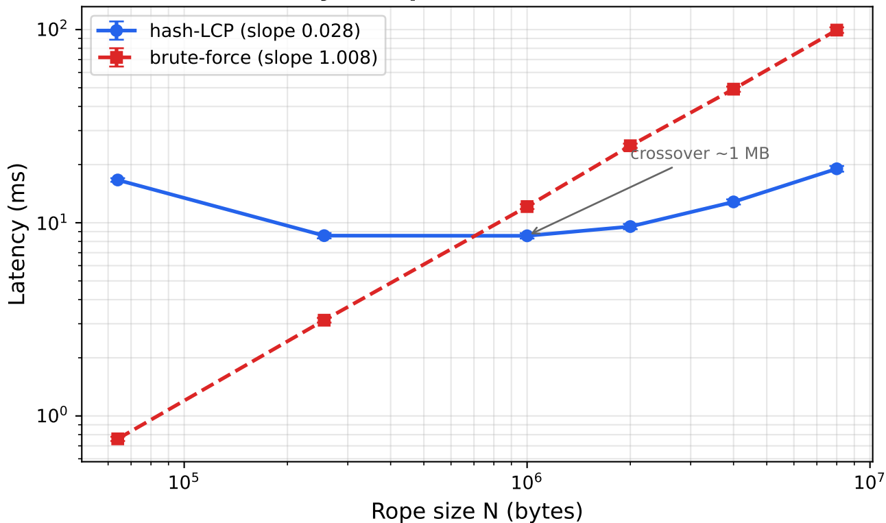
LCP latency vs rope size ( f = 0.5 , n = 9 runs)
