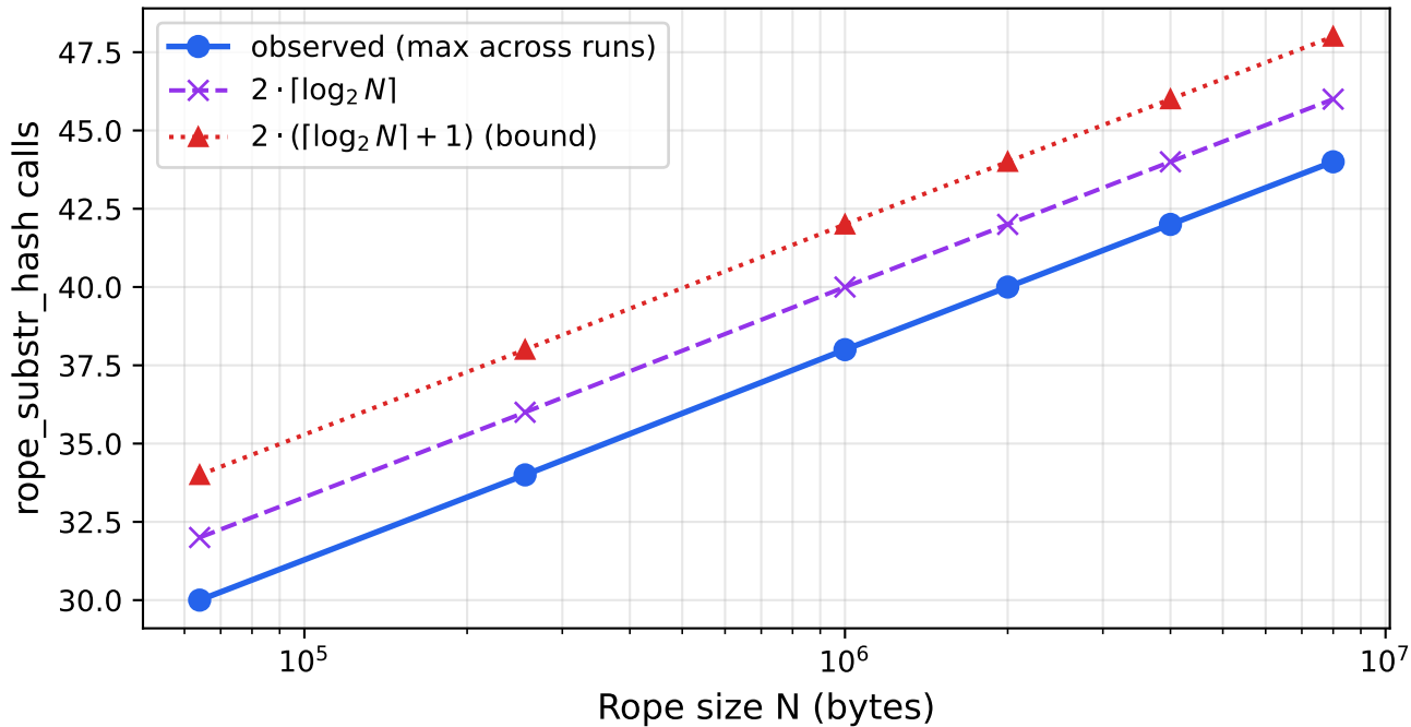
LCP step count vs rope size (f = 0.5)
