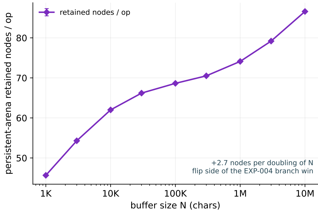
(b) persistent-arena growth under linear churn \sim O(\log N) dead-node retention
