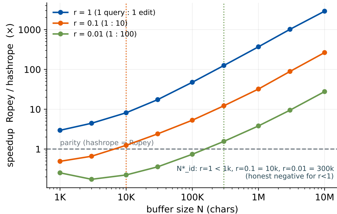
(a) edit+identity speedup vs query density crossover N^*_{id} moves right as queries thin
