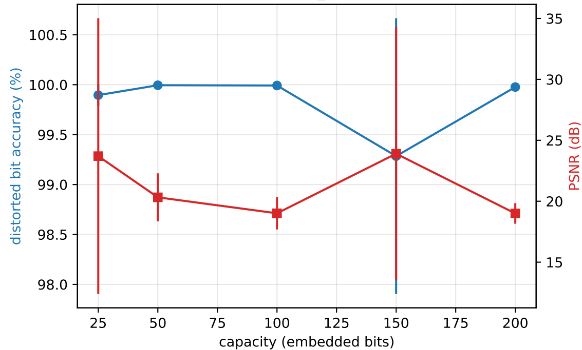
Capacity scaling (cross_channel, distortion)
