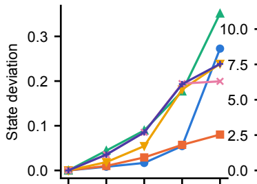
Heat-stress (CBT)
