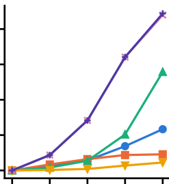
Lying deficit
