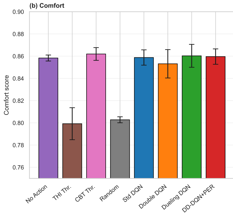
Supplementary: mean \pm SD across 5 independent seeds
