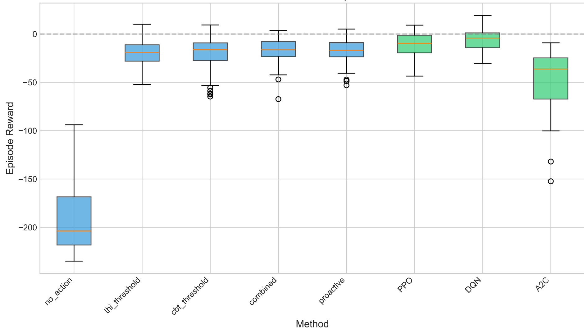
Reward Distribution by Method
