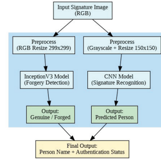
Fig. 5. Multi-Task Parallel Hybrid Architecture Workflow
