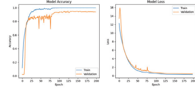
Fig. 10. Training Metrics for CNN on GDPS-100 Dataset
