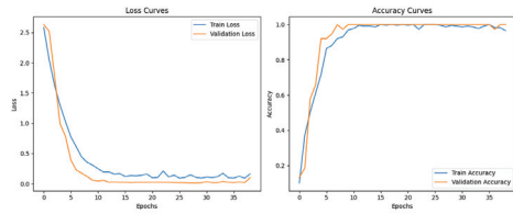
Fig. 6. Training Metrics for CNN on Custom-Collected Dataset
