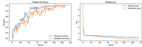
Fig. 8. Training Metrics for InceptionV3 on Custom-Collected Dataset
