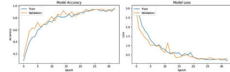
Fig. 12. Training Metrics for InceptionV3 on GDPS-100 Dataset
