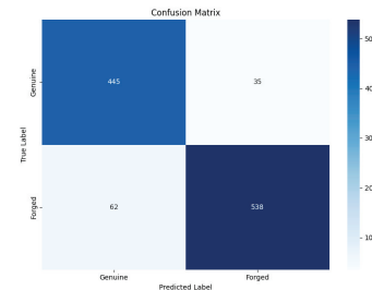
Fig. 13. Confusion Matrix for InceptionV3 on GDPS-100 Dataset
