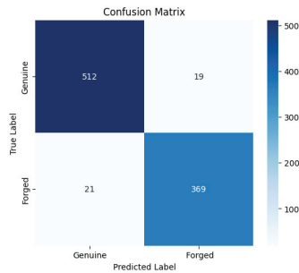
Fig. 9. Confusion Matrix for InceptionV3 on Custom-Collected Dataset
