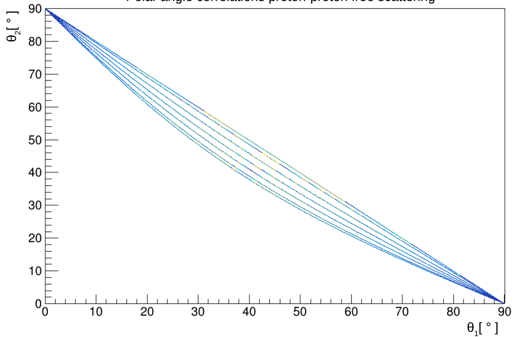
Polar angle correlations proton-proton free scattering
