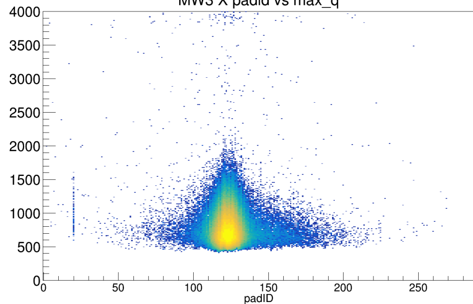
MW3 X padid vs q
