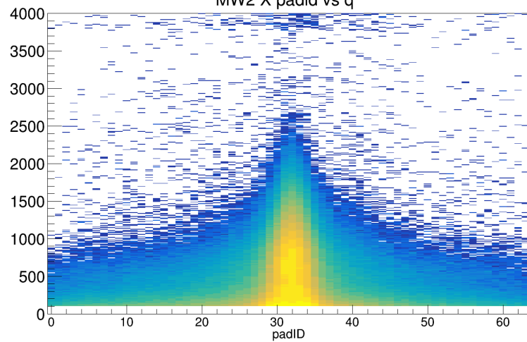
MW2 X padid vs q
