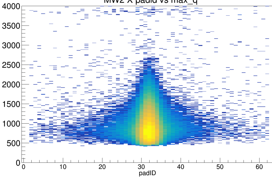
MW2 X padid vs q
