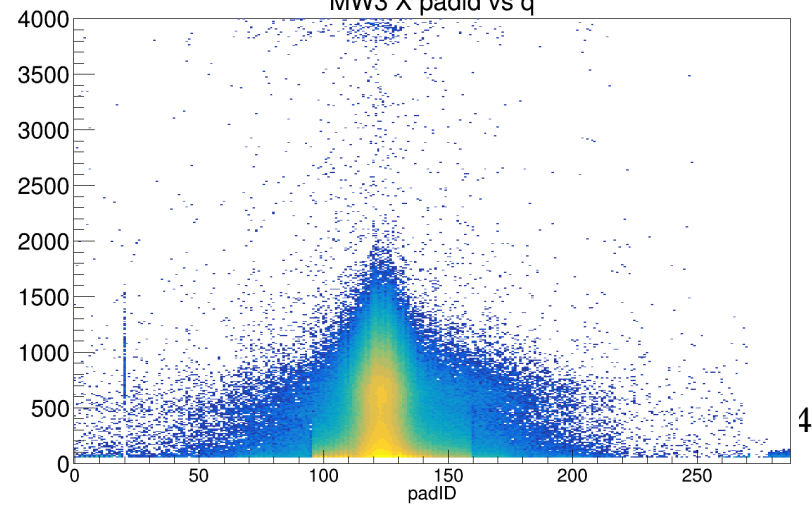
MW3 X padid vs q
