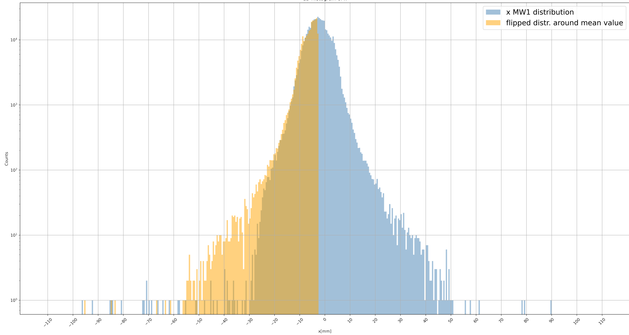
1D Histogram of x
