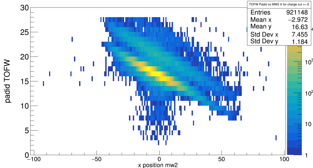
Carbon target, 2cm, 400 AMeV
