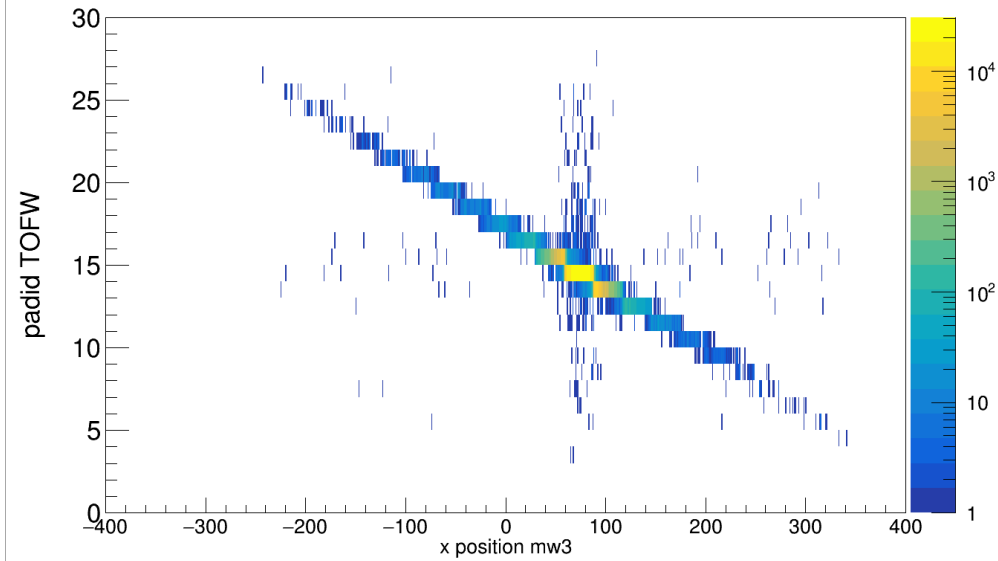
Empty target, 400 AMeV
