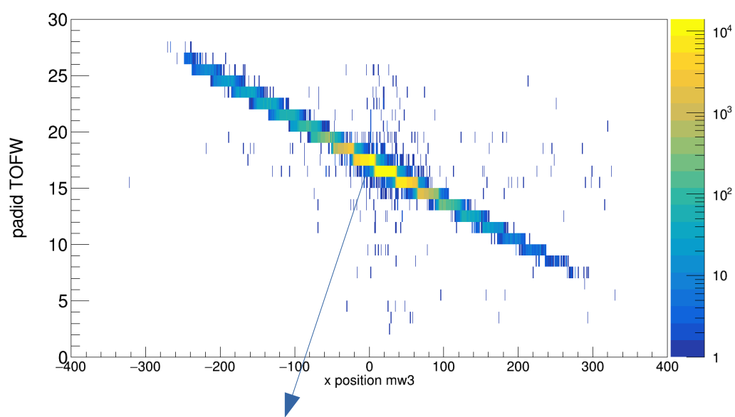
Carbon target, 2cm, 400 AMeV
