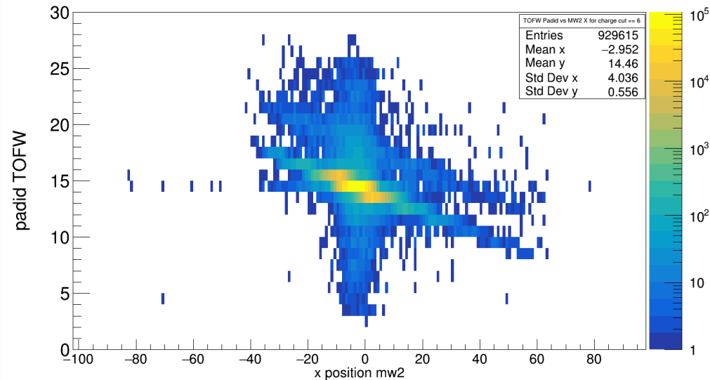
Empty target, 400 AMeV
