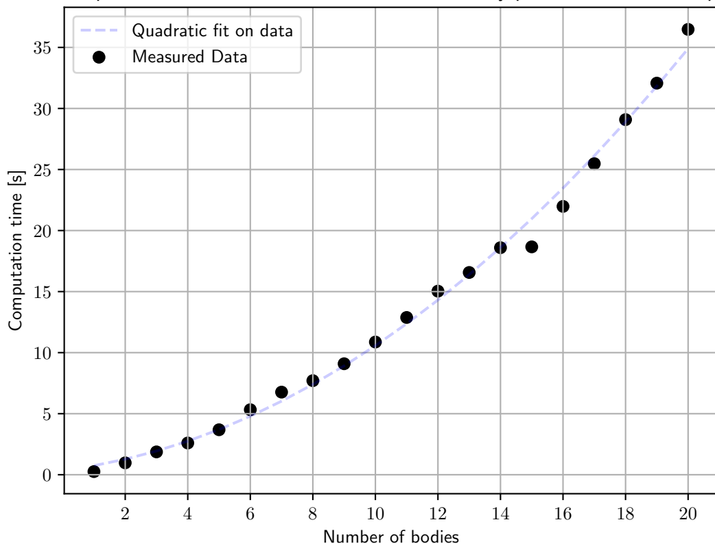
Computation time vs number of bodies for N-body pendulum - RK45 Scipy
