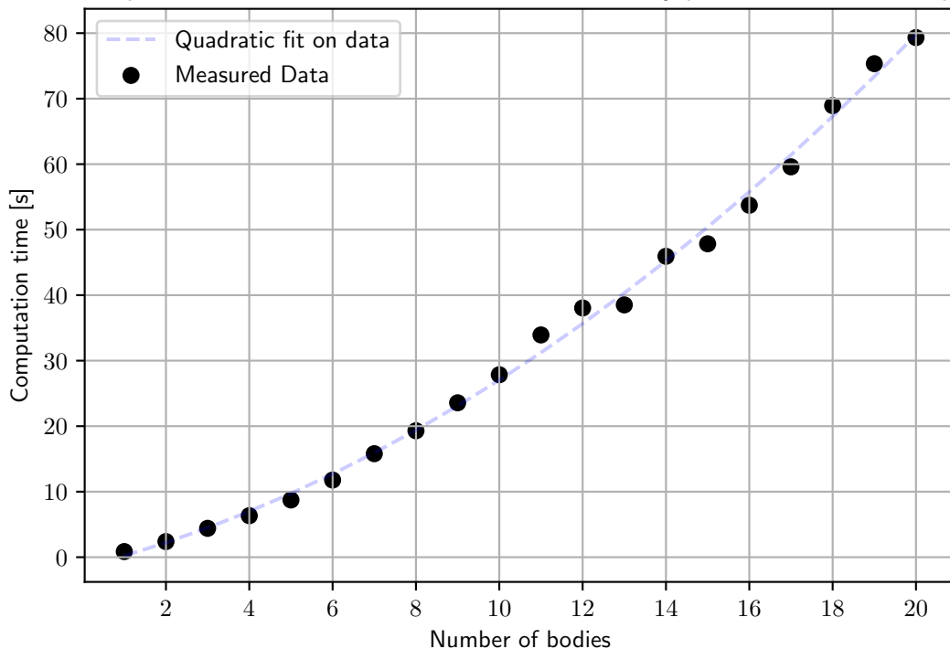
Computation time vs number of bodies for N-body pendulum - RK45 Scipy
