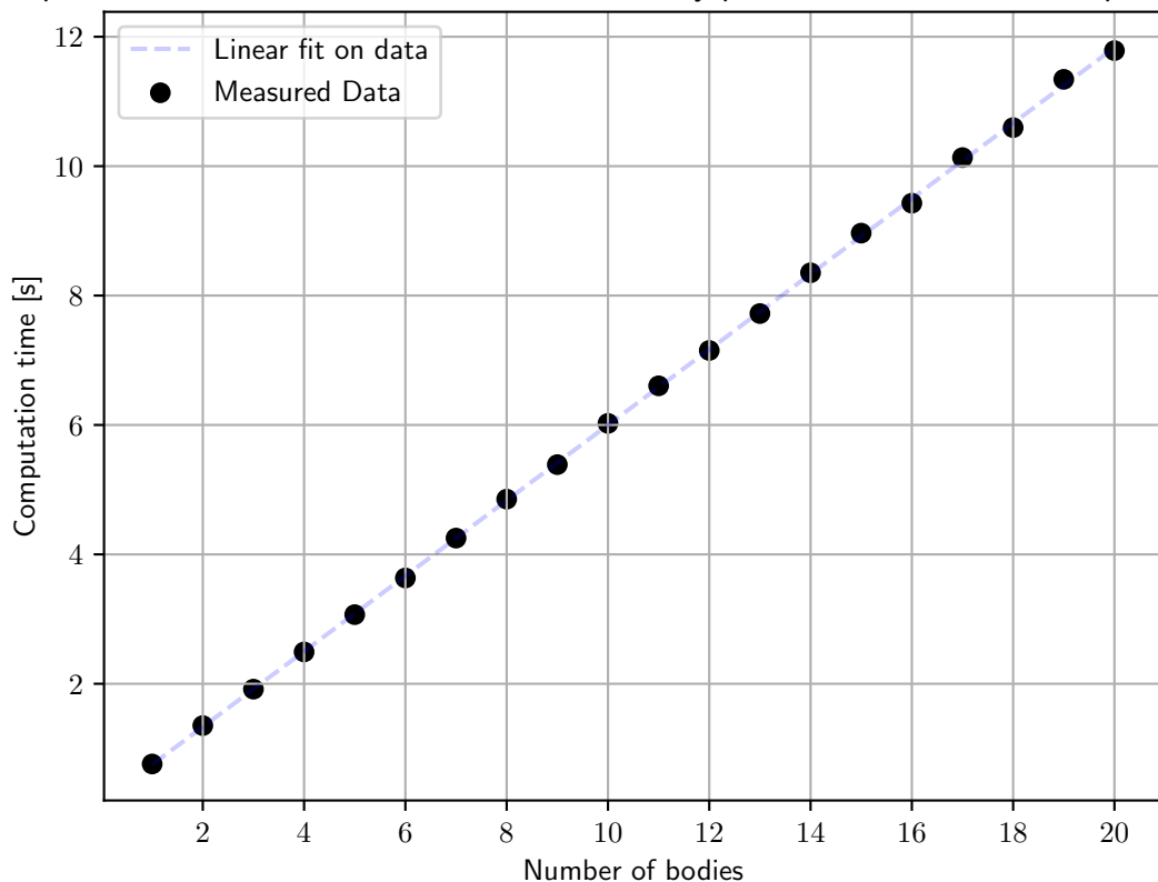
Computation time vs number of bodies for N-body pendulum - RK45 Own implementation
