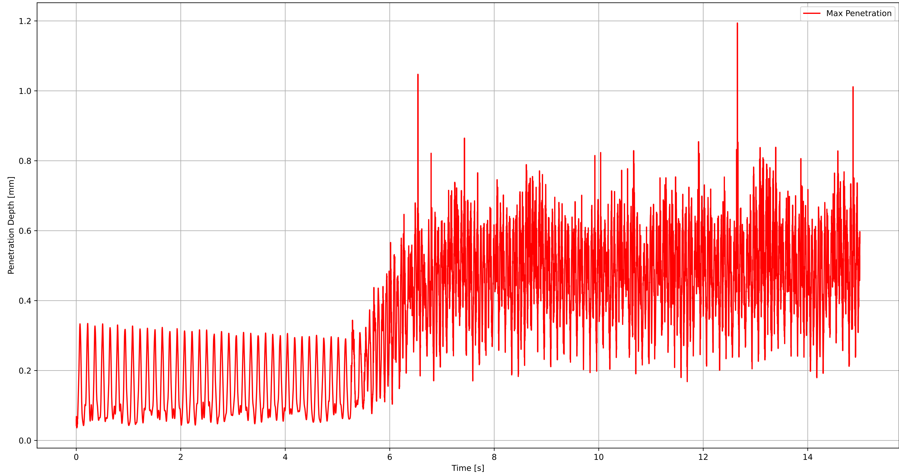
Maximum Joint Penetration into Sprockets over Time
