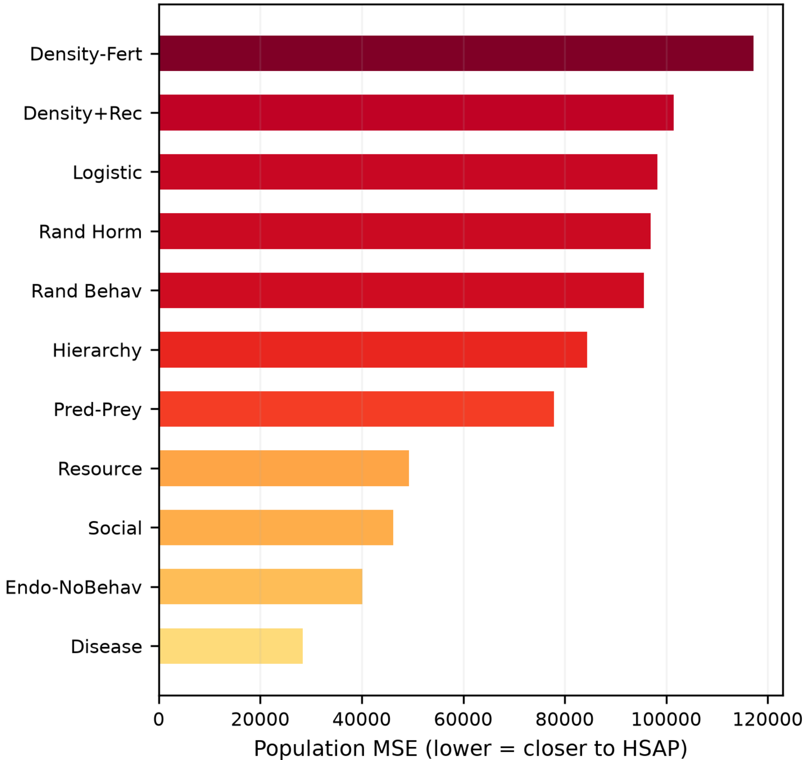
Figure 4a: Null Models — Population Only
