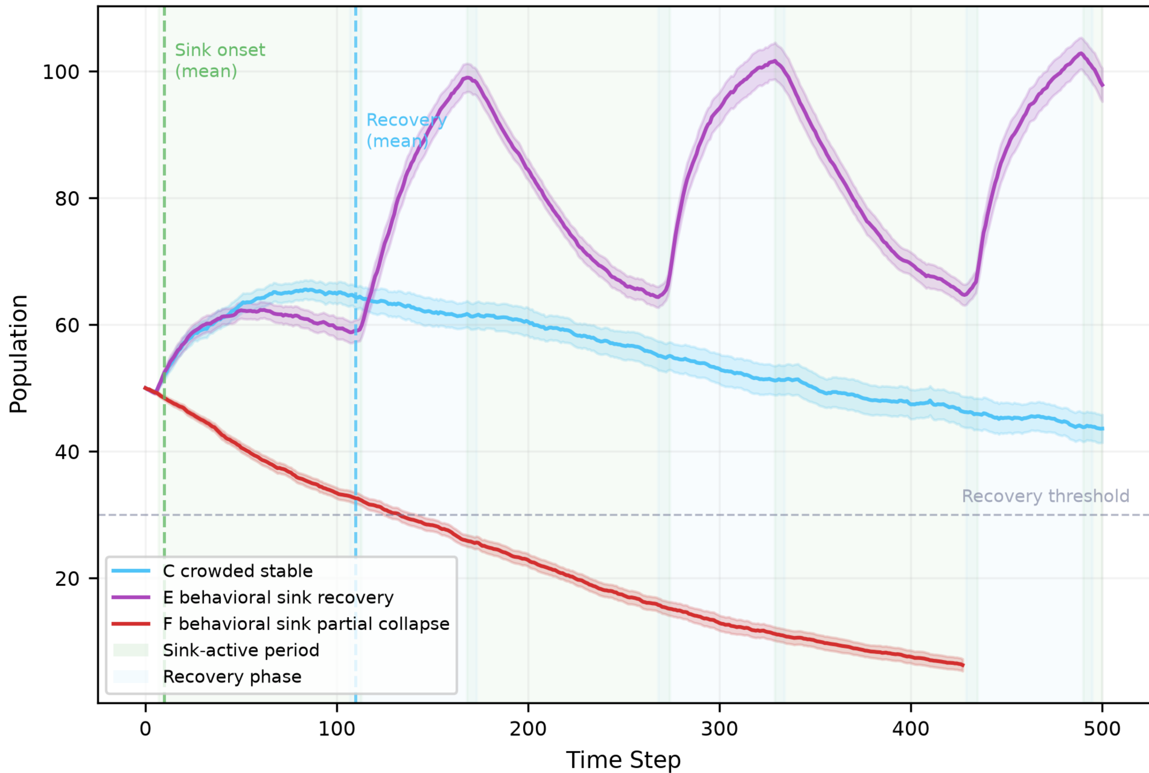
Figure 5: Behavioral Sink Trajectories
