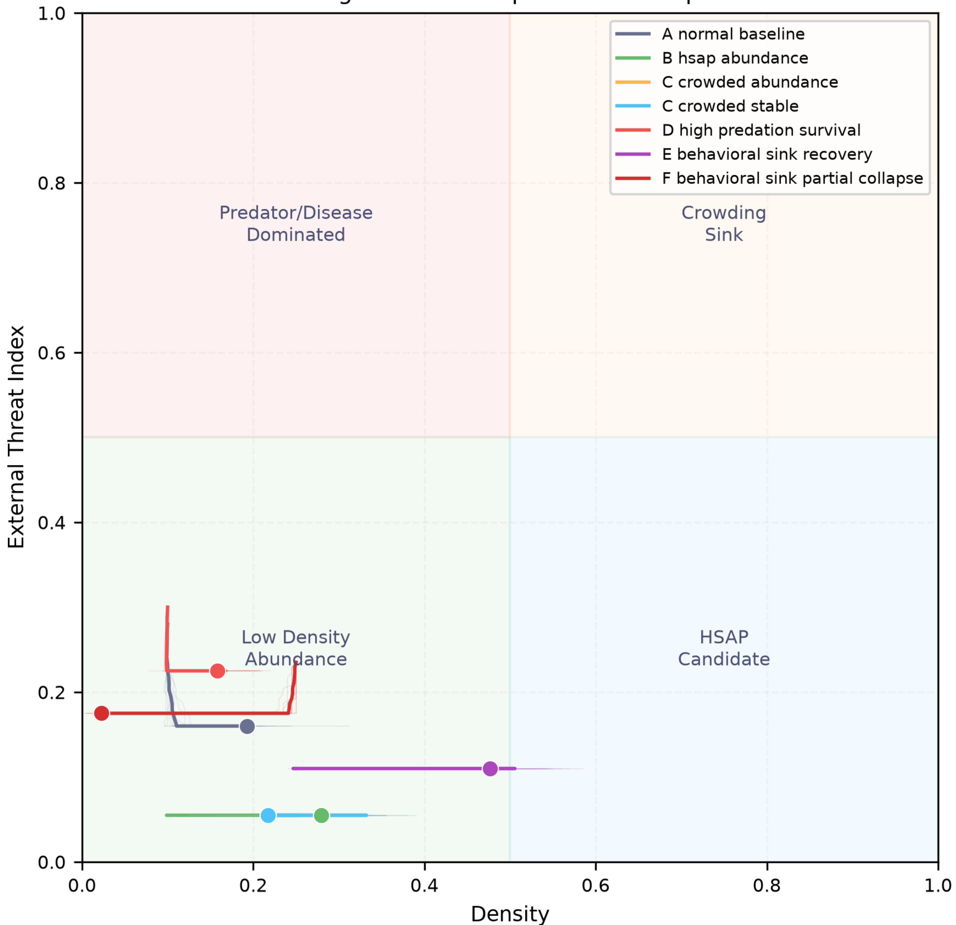
Figure 8: State-Space Phase Map
