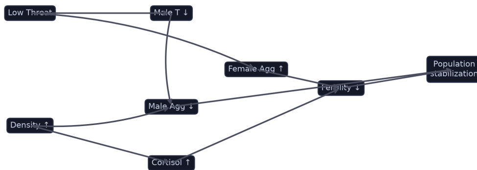
Figure 1: Conceptual structure of the HSAP model. Ecological conditions influence endocrine-linked behavioral state variables, which feed back into fertility, aggression, mortality, and population dynamics.
