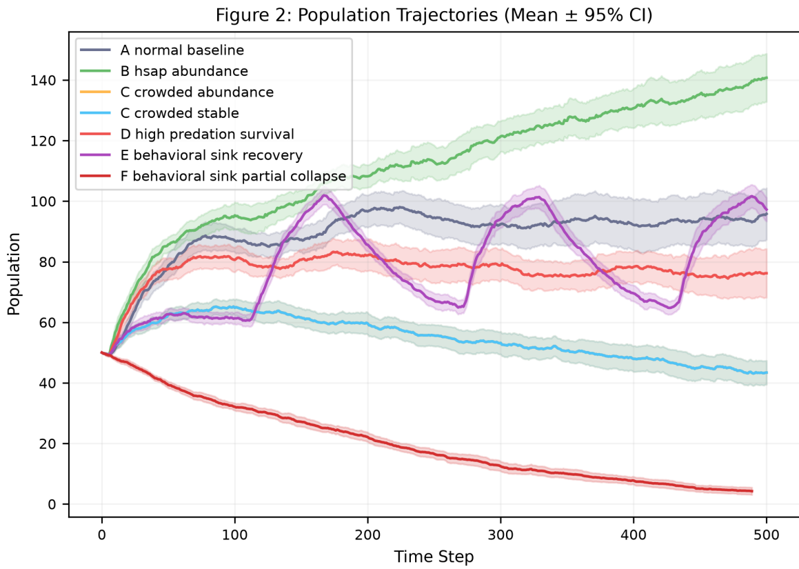
Figure 2: Population trajectories across core HSAP scenarios. Lines summarize the validated simulation runs for baseline, abundance, crowding, and high-predation conditions.
