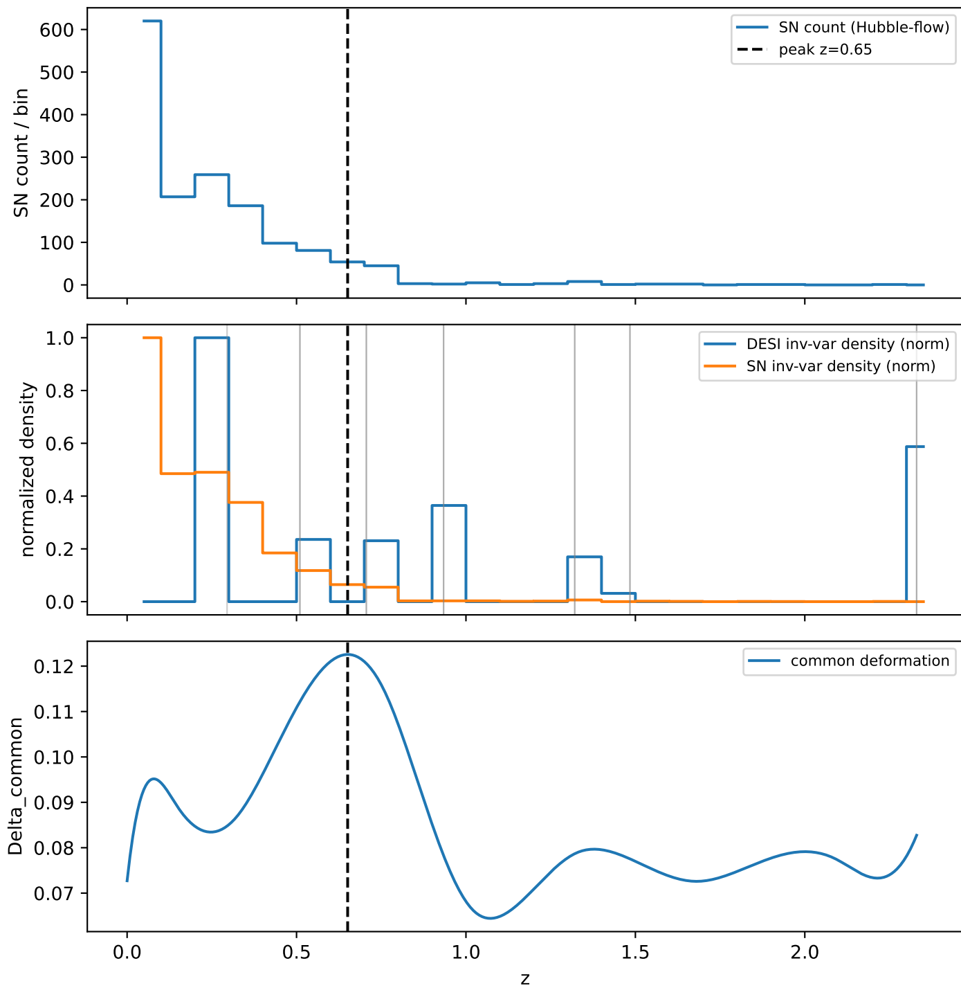
Peak support diagnostic (PEAK_NOT_EXPLAINED_BY_SIMPLE_DATA_DENSITY)
