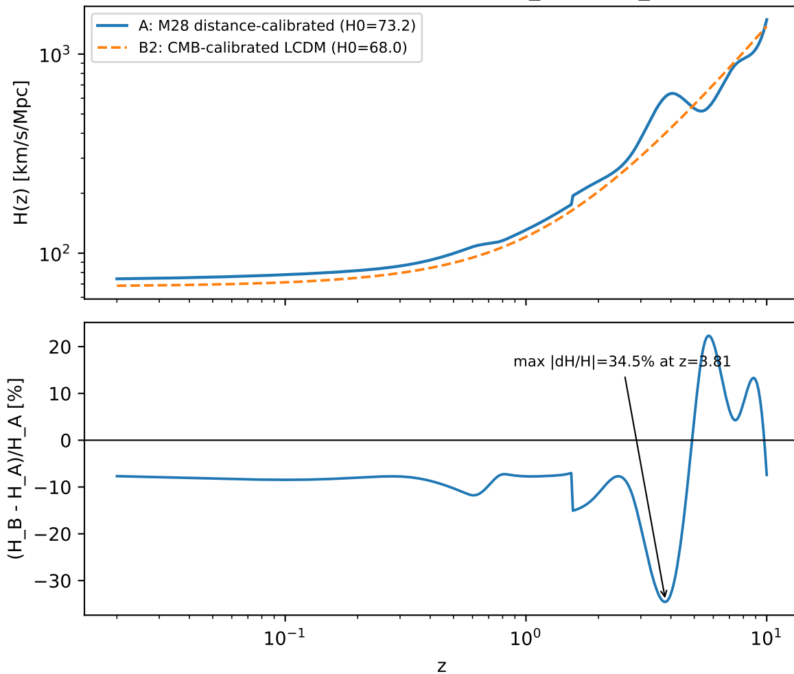
Figure 1: expansion histories H_A(z) vs H_B(z)
