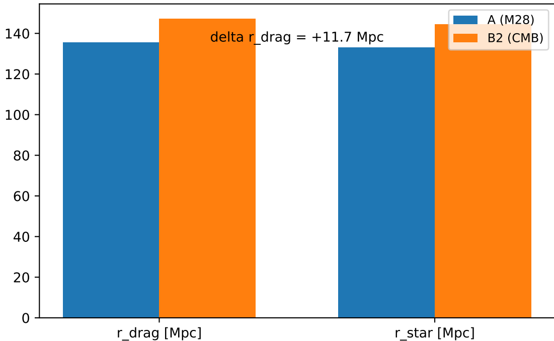
Figure 2: sound horizon r_d(A) vs r_d(B)
