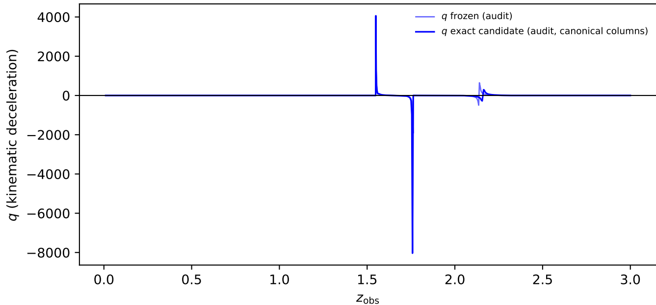
B. Deceleration diagnostic from audit epoch curves ( n_{\text{stable}}=0 )
