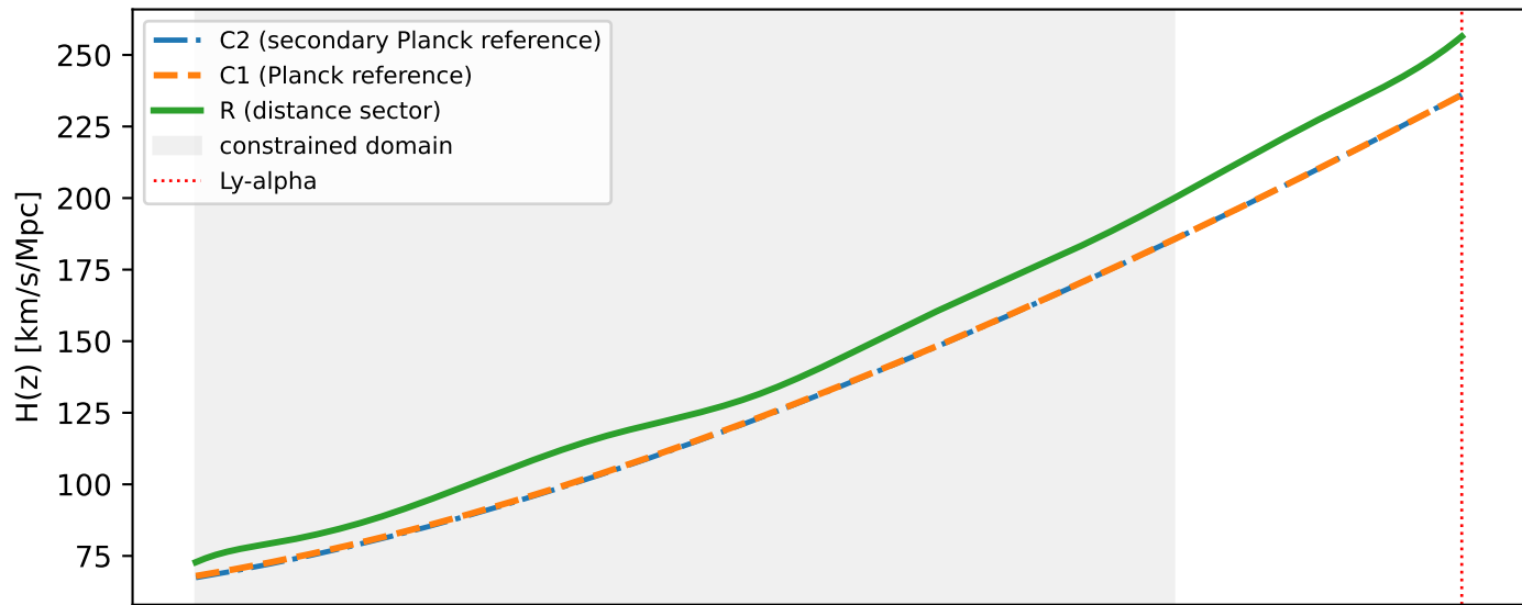
Frozen endpoint histories
