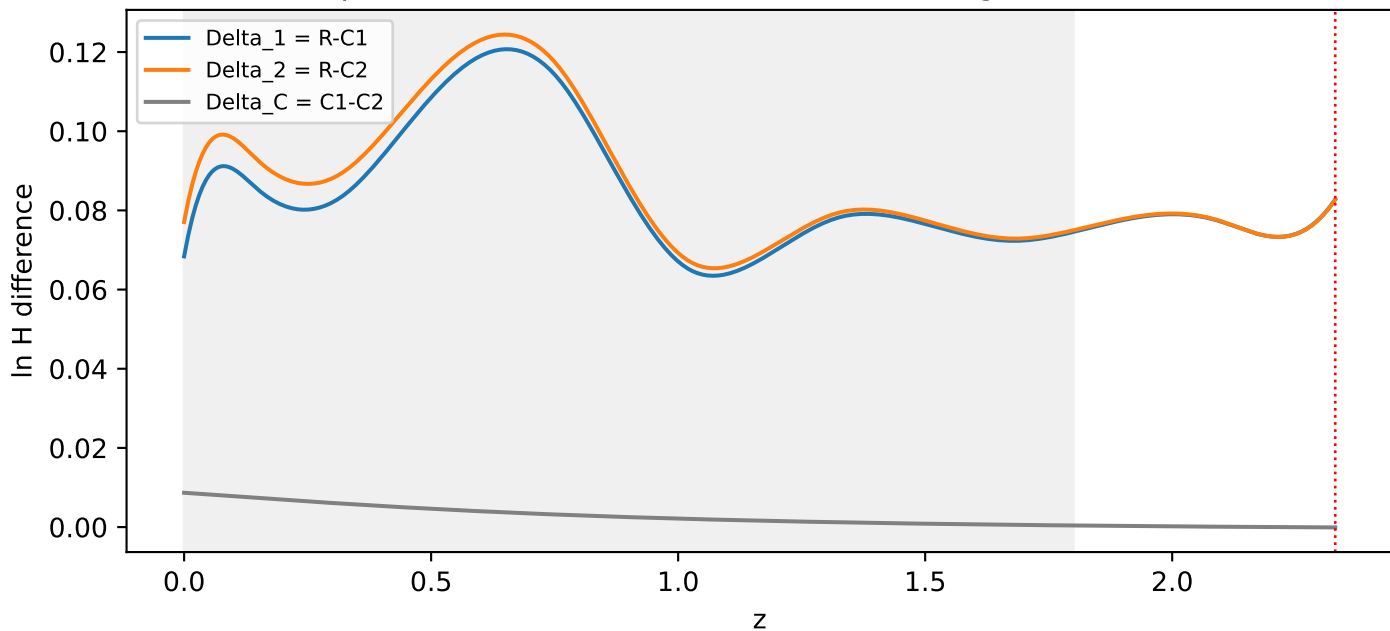
Endpoint differences (C1-C2 an order of magnitude smaller)
