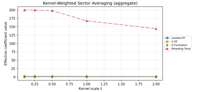
FIG. 9: Kernel-weighted sector averaging under unobserved-sector mixing. As \ell increases, aggregate parameters interpolate between the x_0 basin values and the global average.
