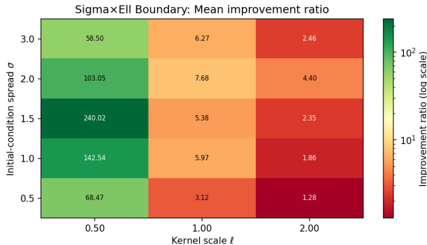
FIG. 7: Mean improvement ratio (global KL / ISR KL) across the sigma-ell grid. All non-degenerate cells ( \ell \geq 0.50 ) exceed 1.
