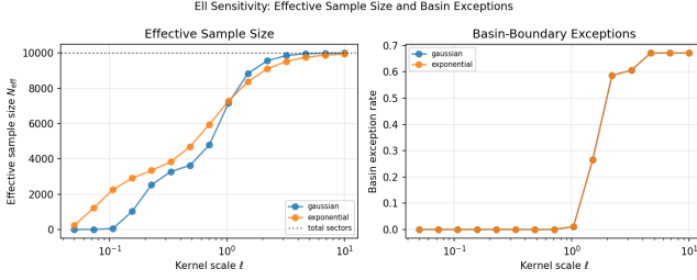
FIG. 10: Effective sample size N_{\text{eff}} and basin exception rate vs. \ell . The sweet spot lies where N_{\text{eff}} is large enough for statistical power but basin exceptions remain below 30%.
