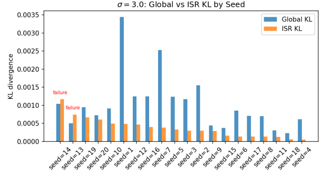
FIG. 8: KL divergence at \sigma = 3.0 for global census and ISR by seed. Two seeds (13 and 14) show ISR above global.
