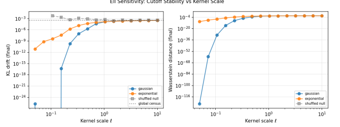
FIG. 6: KL drift and Wasserstein distance vs. kernel scale \ell . The black dotted line is the global-census baseline; the gray dashed line is the shuffled null control.
