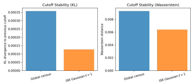
FIG. 3: KL divergence and Wasserstein distance for global census and ISR (Gaussian \ell = 1 ) at N = 10,000 . ISR reduces both metrics.
