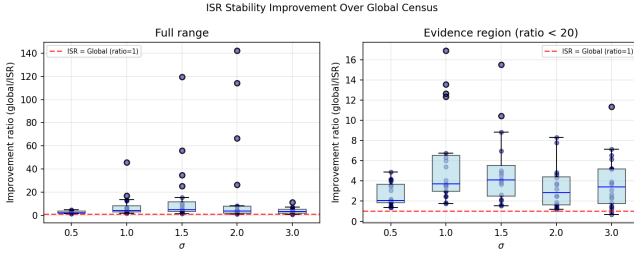
FIG. 4: Improvement ratio D_{\text{KL}}^{\text{global}}/D_{\text{KL}}^{\text{ISR}} by \sigma . Points above 1 (dashed red line) indicate ISR outperforms global. Boxes show quartiles across 20 seeds per \sigma .
