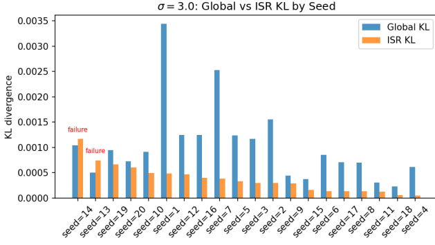
FIG. 10: KL divergence at \sigma = 3.0 for global census and ISR by seed. Two seeds (13 and 14) show ISR above global.
