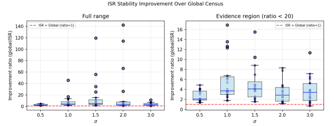
FIG. 4: Improvement ratio D_{\text{KL}}^{\text{global}}/D_{\text{KL}}^{\text{ISR}} by \sigma . Points above 1 (dashed red line) indicate ISR outperforms global. Boxes show quartiles across 20 seeds per \sigma .
