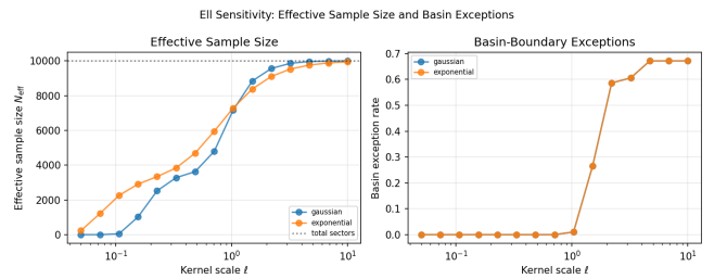
FIG. 10: Effective sample size N_{\text{eff}} and basin exception rate vs. \ell . The sweet spot lies where N_{\text{eff}} is large enough for statistical power but basin exceptions remain below 30%.
