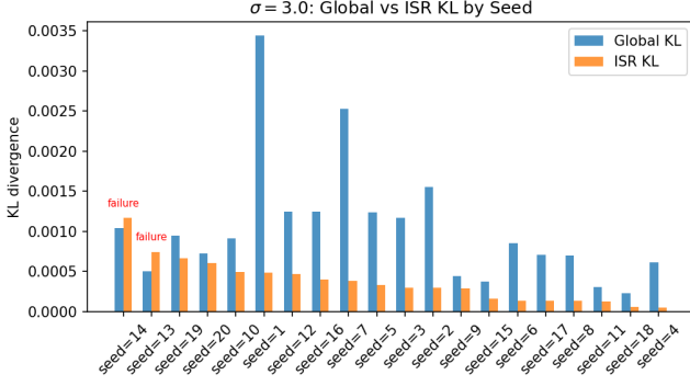
FIG. 8: KL divergence at \sigma = 3.0 for global census and ISR by seed. Two seeds (13 and 14) show ISR above global.
