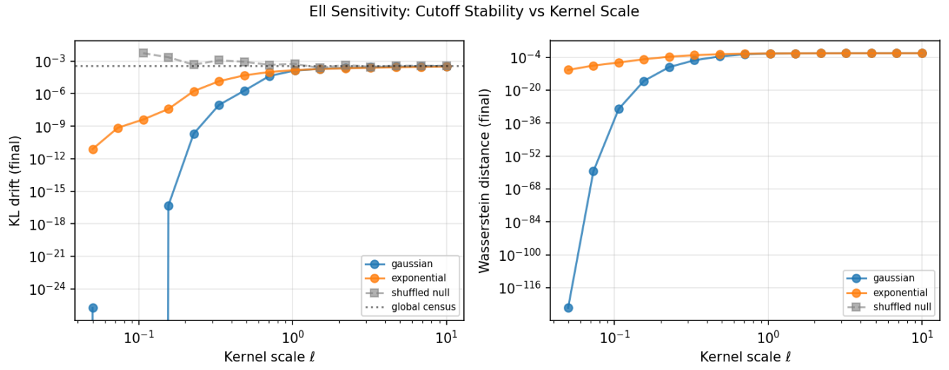
FIG. 6: KL drift and Wasserstein distance vs. kernel scale \ell . The black dotted line is the global-census baseline; the gray dashed line is the shuffled null control.
